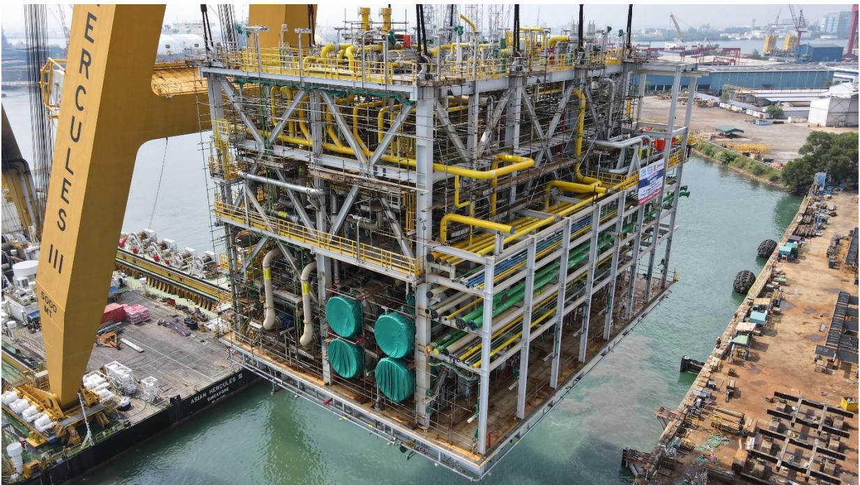
Inlet Separation / Oil Separation and Desalting Flare System Module
